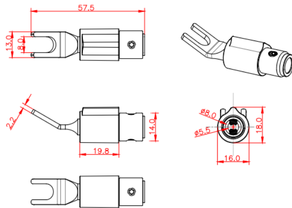
Furutech Ethereal FT-211 Spade Terminals
